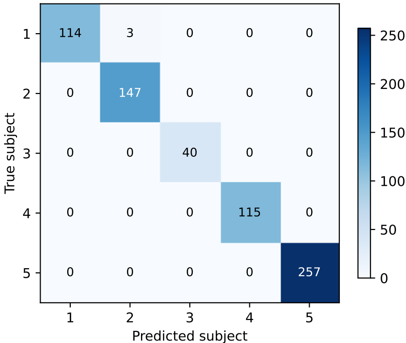
Confusion matrix after PCA (N=8, acc 0.996)
